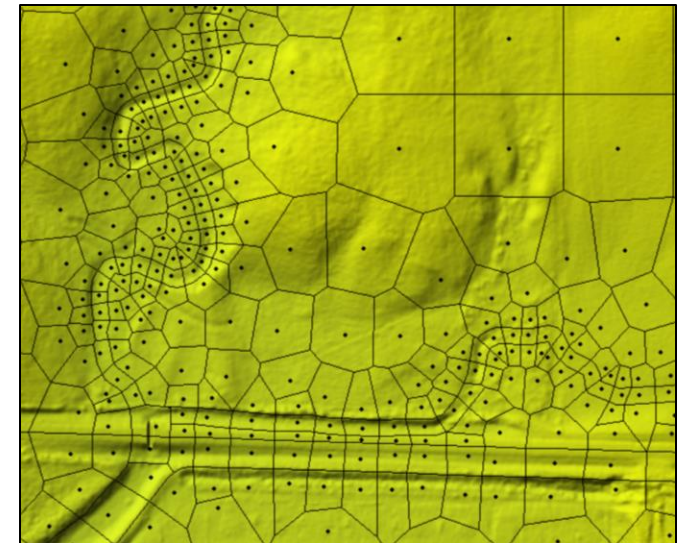
Refined Mesh
