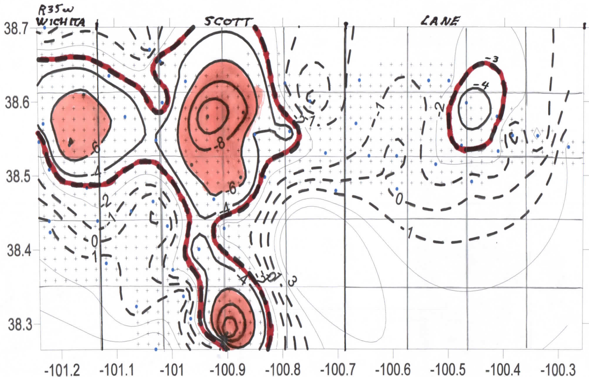
10-Year (Jan2012 to Jan2022) Observation Well Water Level Change with Section centers (per 10 yrs, not per yr). Observation wells in blue.
