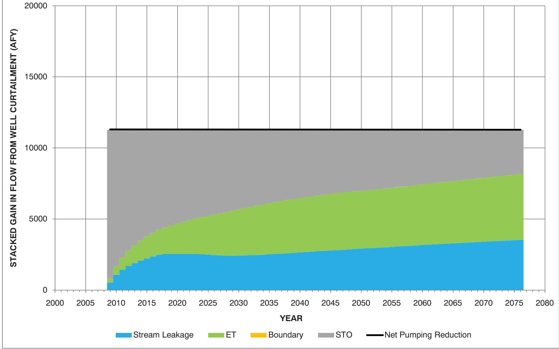
FIGURE 65 ILLUSTRATIVE SOURCE OF WATER TO WELLS IN RESPONSE TO MANAGEMENT ACTION (BASELINE B')
