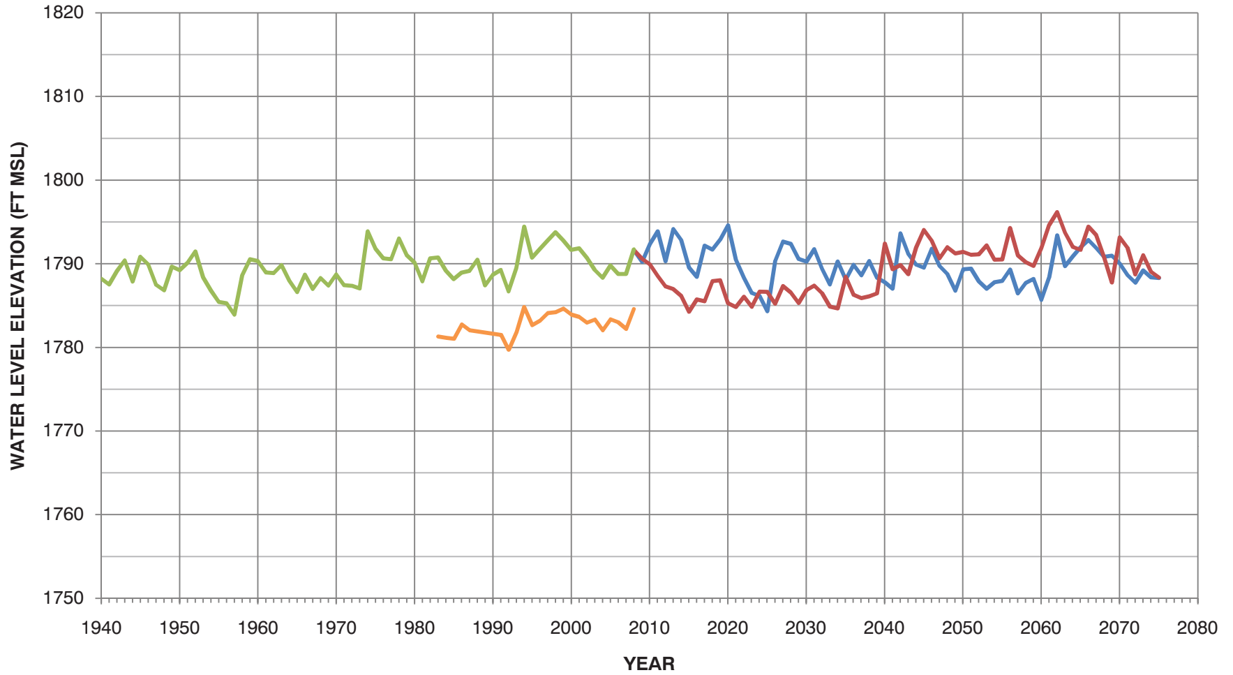
FIGURE 58 BASELINE A AND B HYDROGRAPH OF WELL WQ-17 (MAP ID 2)
