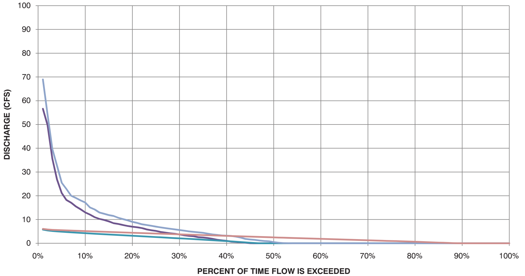
FIGURE 70 DURATION CURVE OF MANAGEMENT ACTION EFFECT AT RATTLESNAKE CREEK NEAR MACKSVILLE, KS
