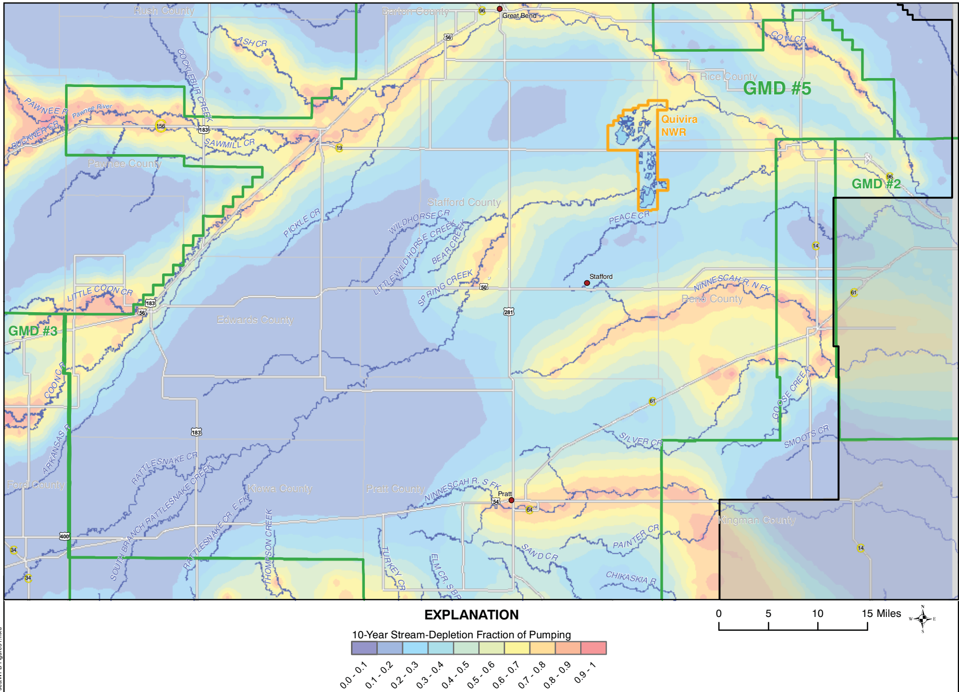
FIGURE 51. Ten-Year Stream-Depletion Fraction of Pumping (From Year 2020 Condition to Year 2030)
