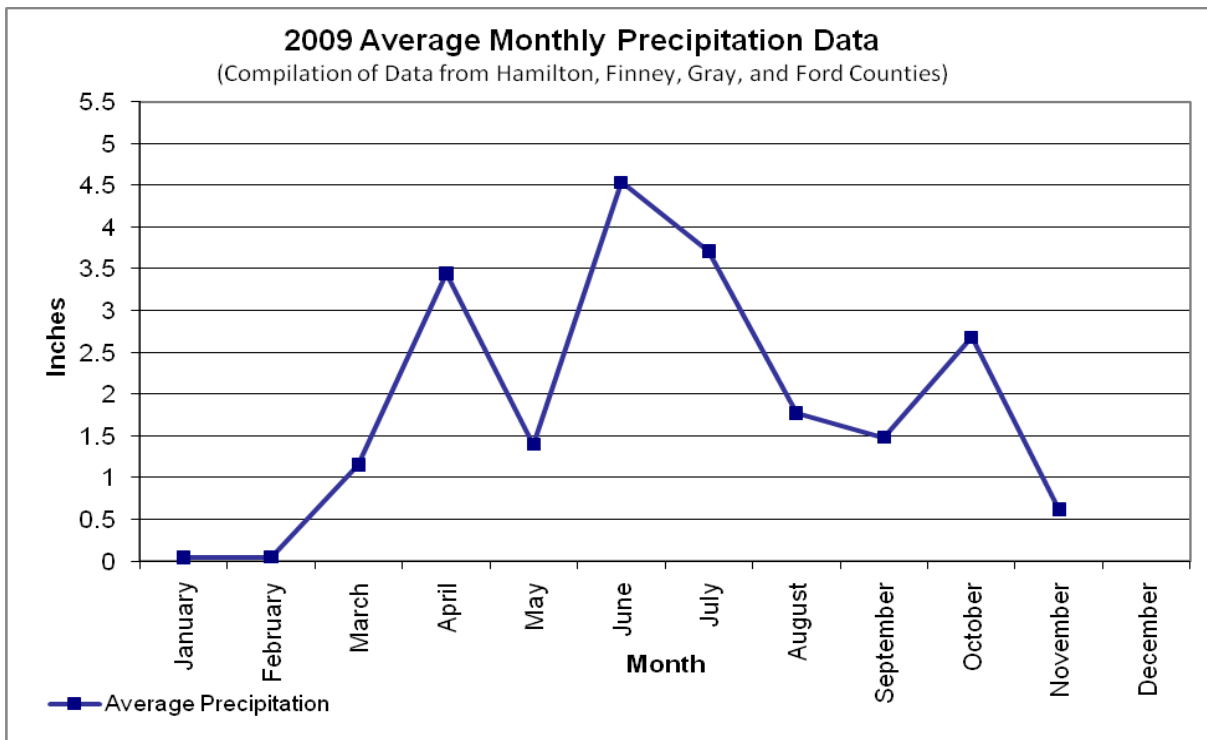
Figure 3: Monthly Average Precipitation in Upper Arkansas Subbasin for 2009
