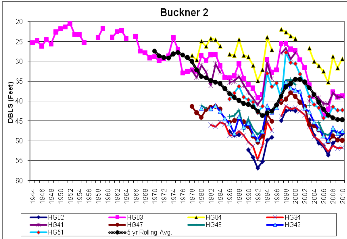
Figure 10: Monitoring well levels in Buckner 2
