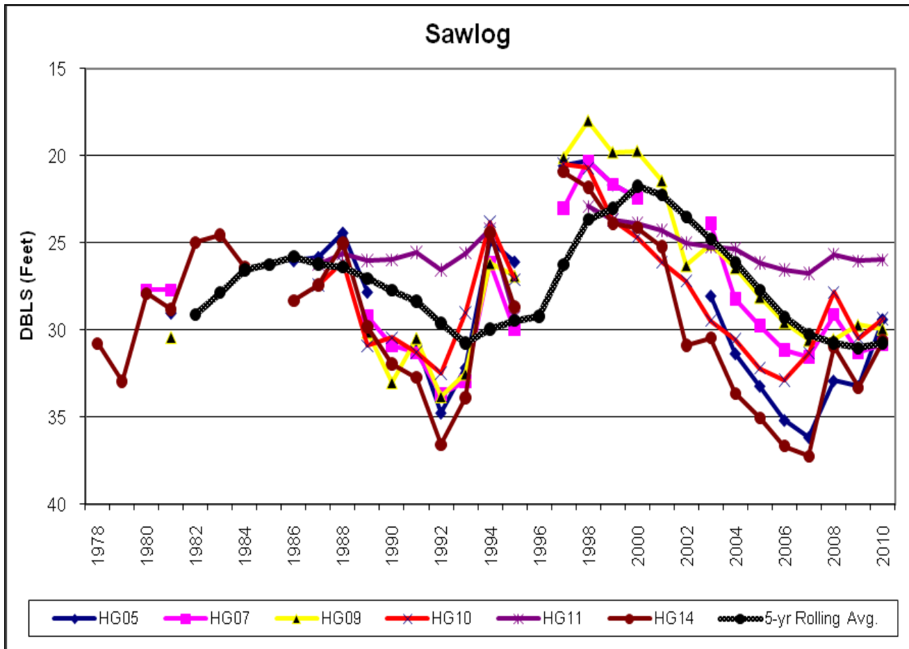
Figure 17: Monitoring well levels Sawlog
