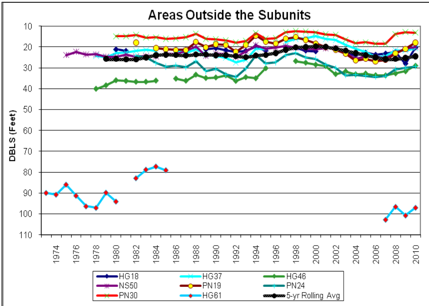
Figure 19: Monitoring well levels outside defined subunits.
