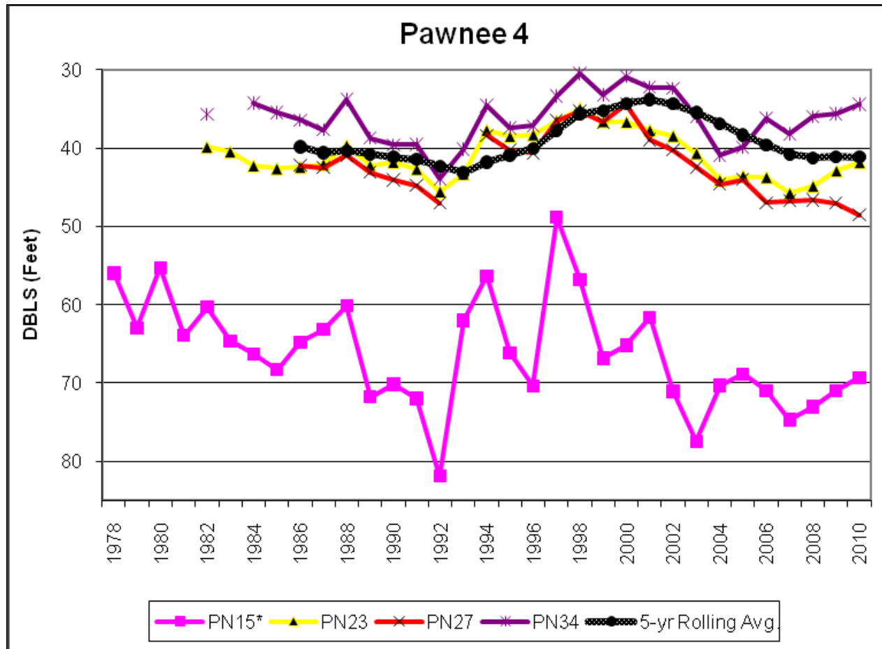
Figure 14: Monitoring well levels Pawnee 4
