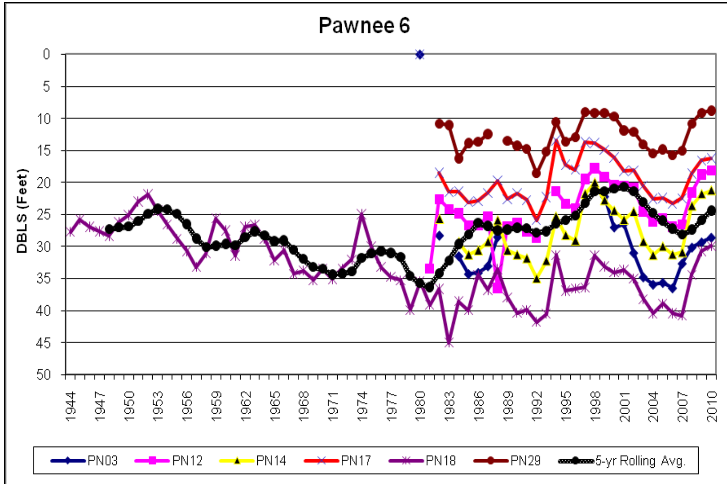
Figure 16: Monitoring well levels Pawnee 6
