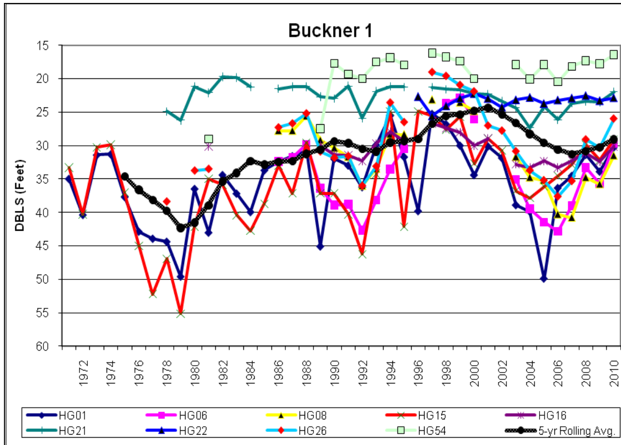
Figure 9: Monitoring well levels in Buckner 1
