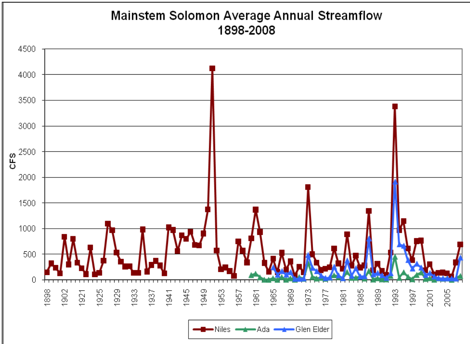
Figure 5: Average Annual Streamflow at USGS Gages 1898-2008 NOTE: There is no data for 1903-1917
