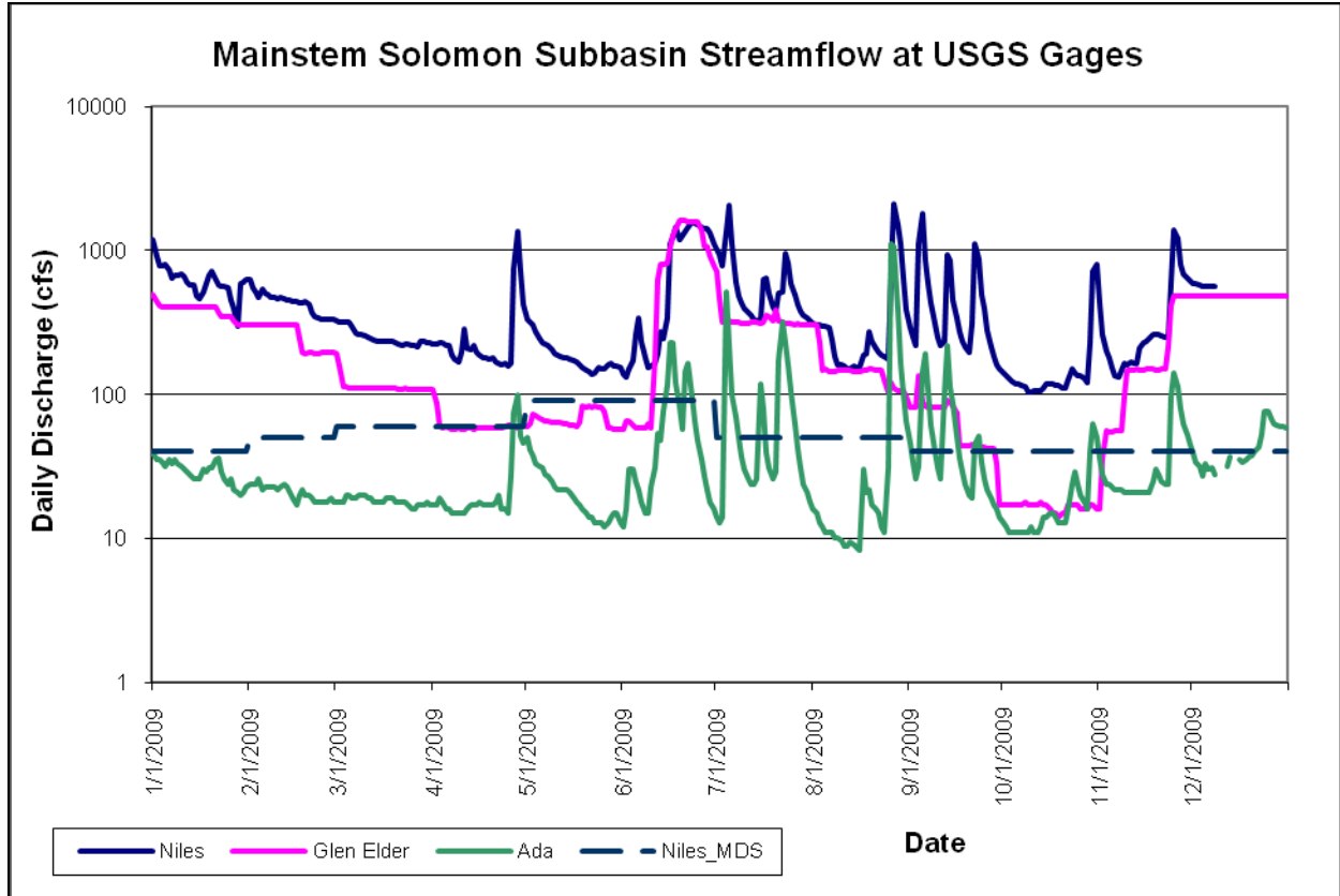
Figure 6: Daily Streamflow and MDS for Niles 2009
