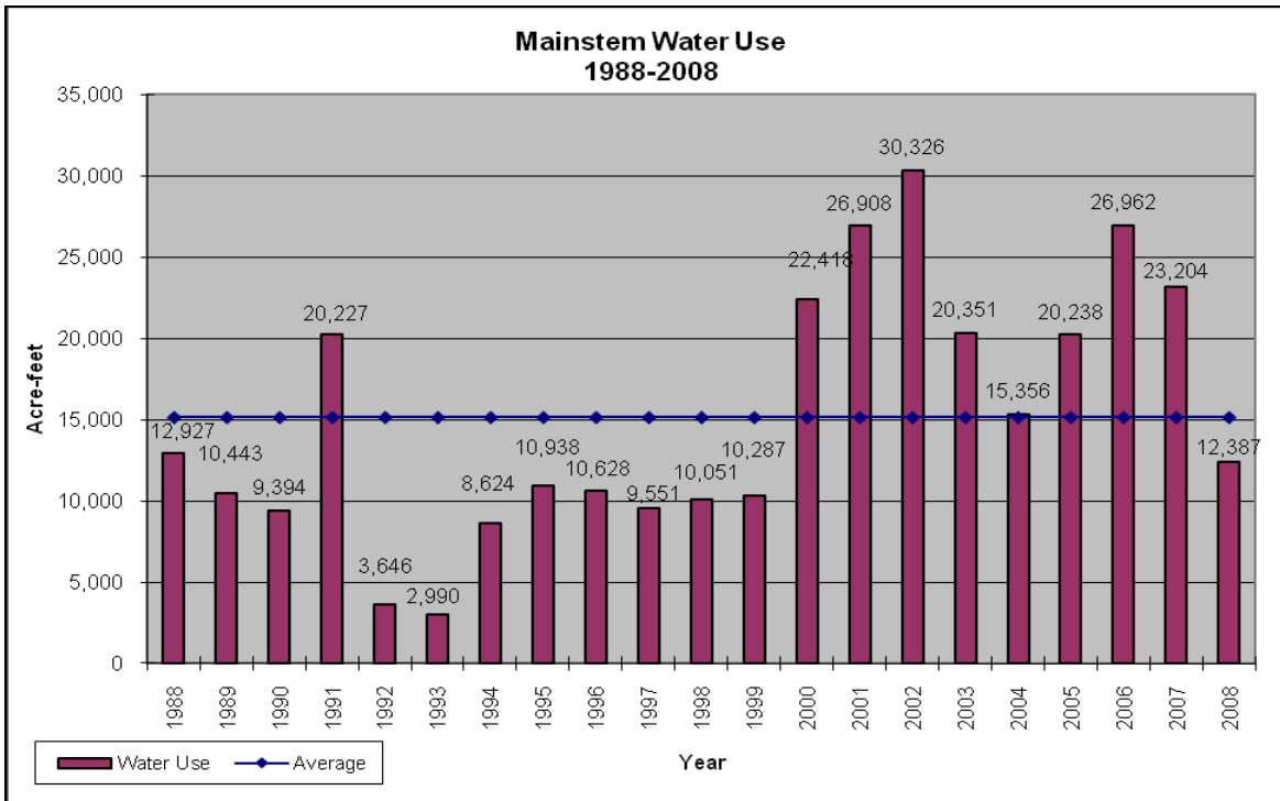
Figure 11: Ground and surface water use by year
