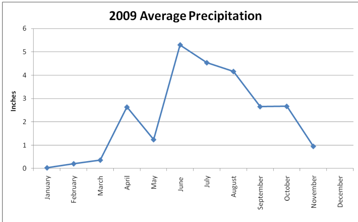
Figure 3: 2009 Monthly Average Precipitation (December data not available)
