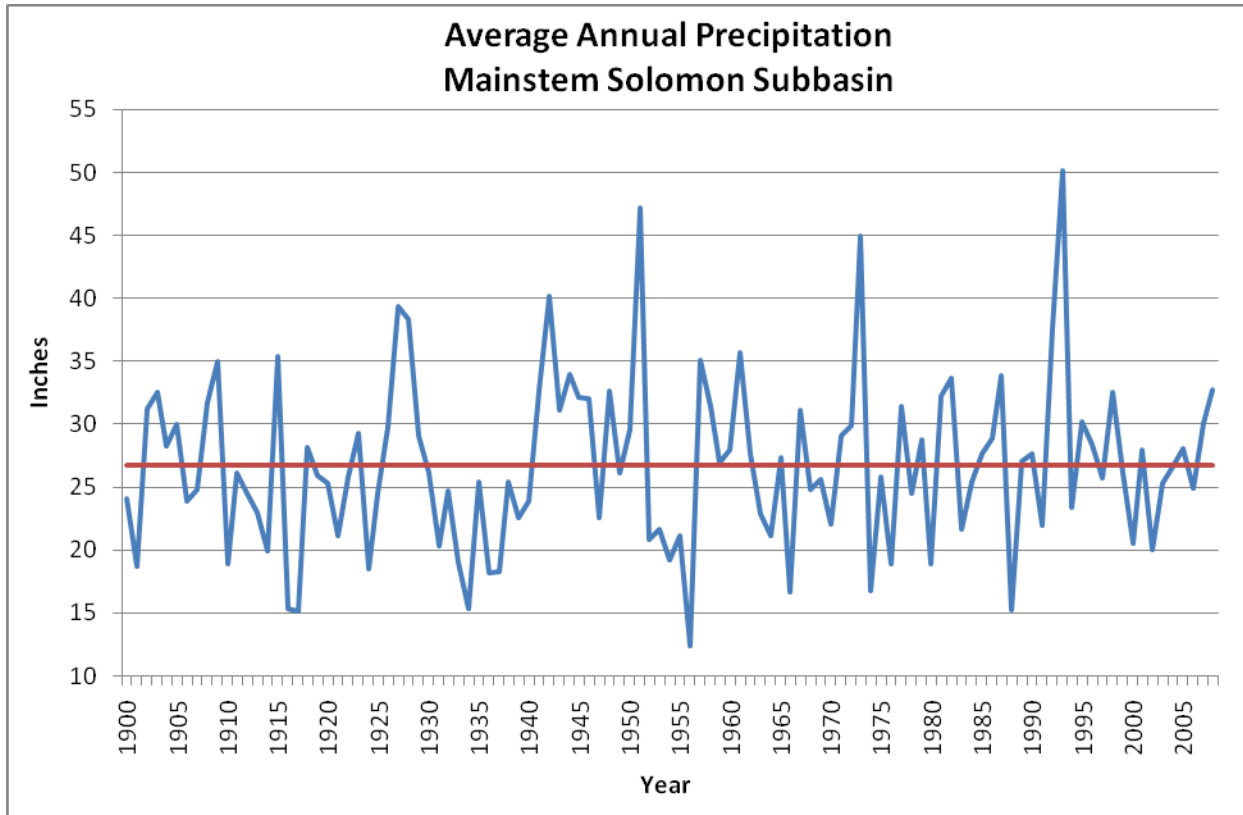
Figure 2: Mainstem Solomon Subbasin precipitation 1900-2008
