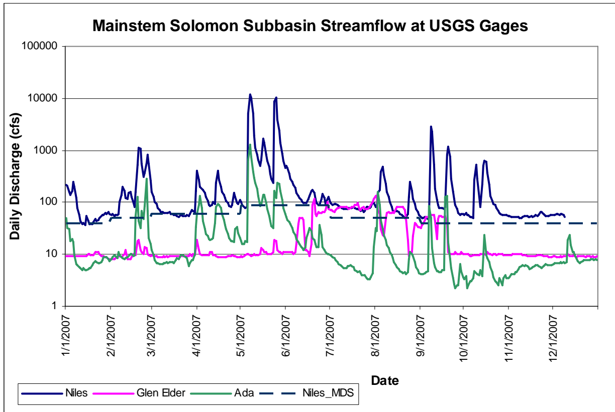
Figure 6: Daily Streamflow and MDS for Niles 2007
