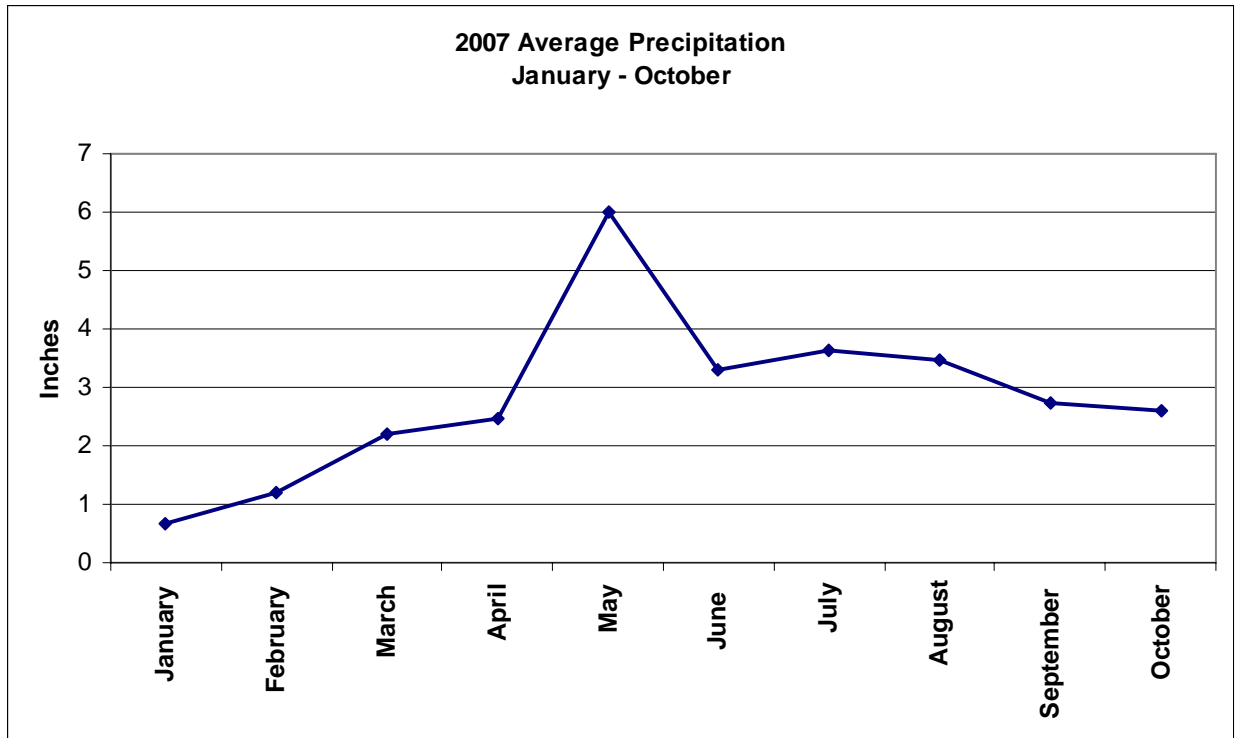
Figure 3: 2007 Monthly Average Precipitation (November and December data not available)
