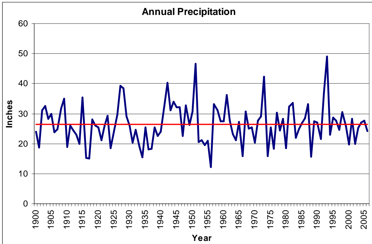
Figure 2: Mainstem Solomon Subbasin precipitation 1900-2006
