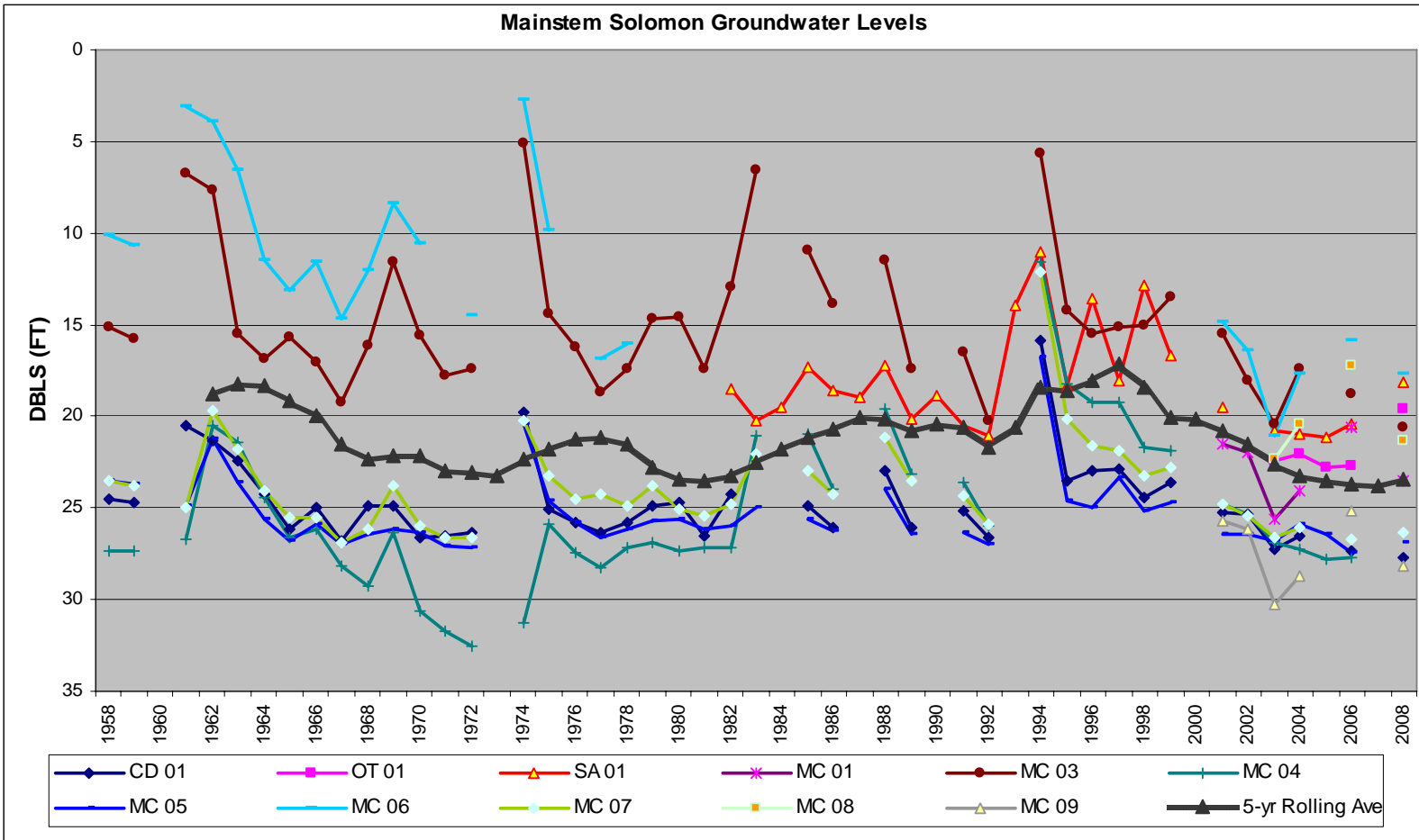
Figure 9: Monitoring wells located in the Mainstem Solomon Subbasin
